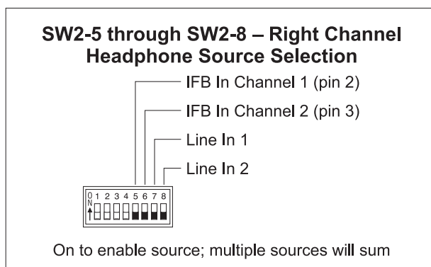
Figure 7. Left and right channel headphone source selection settings
