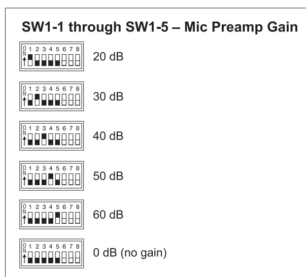
Figure 4. Microphone preamplifier gain switch settings
