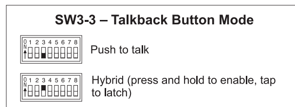
Figure 10. Talkback output button mode settings
